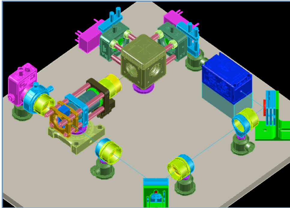
Figure 3. Automatically generated BeamWise 3D CAD rendered drawing of the flow cytometer optofluidic bench.
